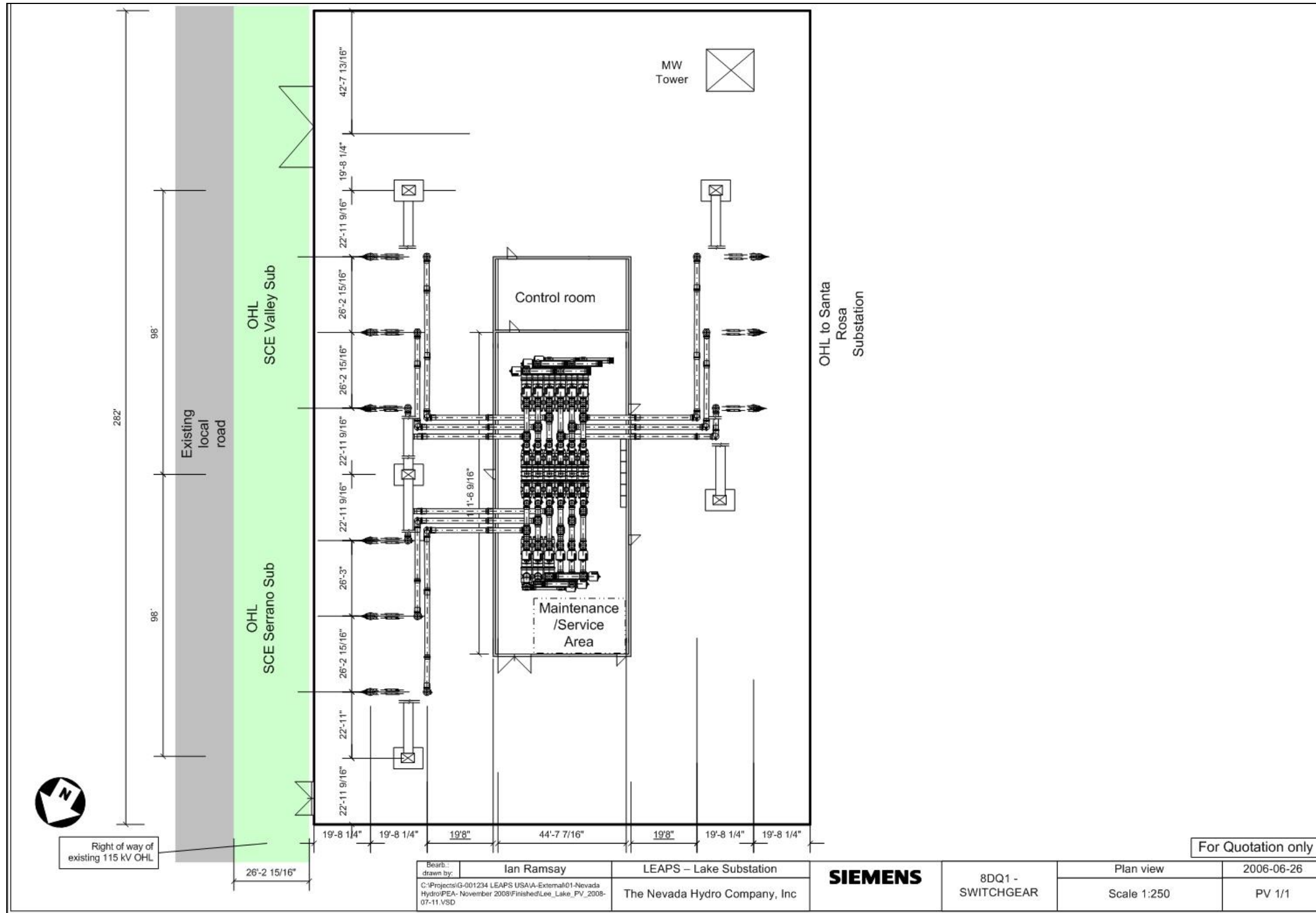
Lake 500kV Switchyard – Conceptual Plan Layout Source: Siemens Power Transmission & Distribution
