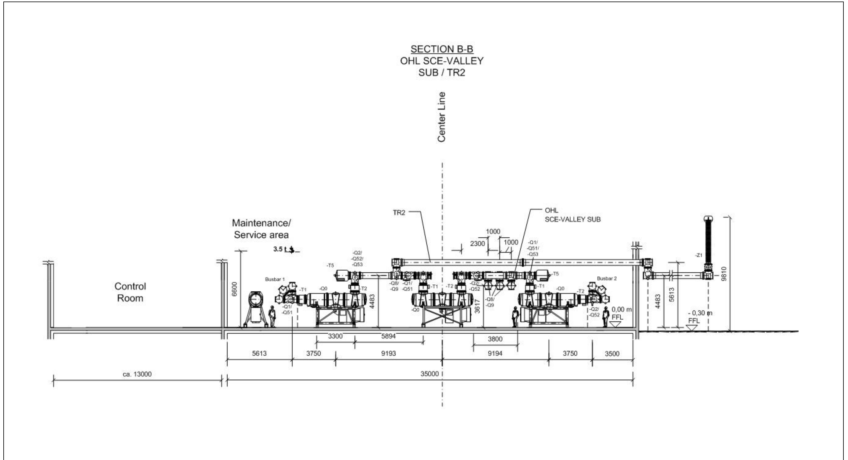
Lake 500 kV Switchyard – Conceptual Elevation Drawings (2 of 3) Source: Siemens Power Transmission & Distribution
