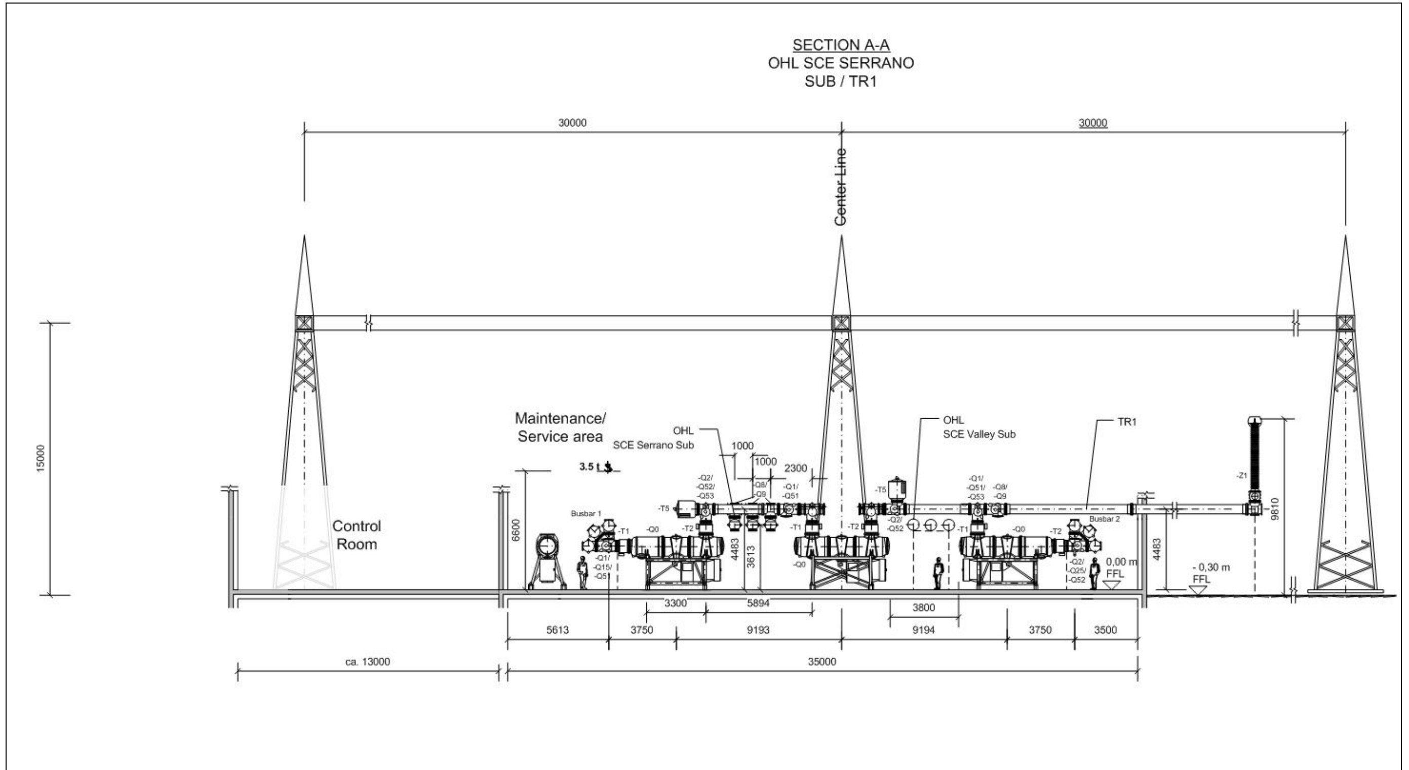
Lake 500 kV Switchyard – Conceptual Elevation Drawings (1 of 3)
