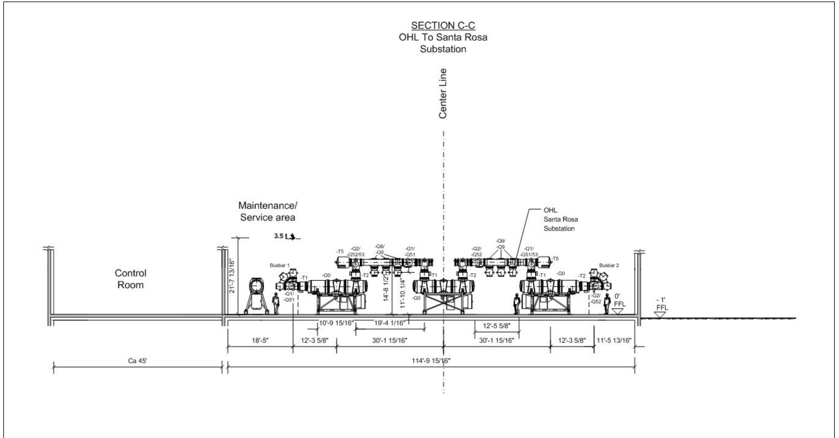
Lake 500 kV Switchyard – Conceptual Elevation Drawings (3 of 3)
