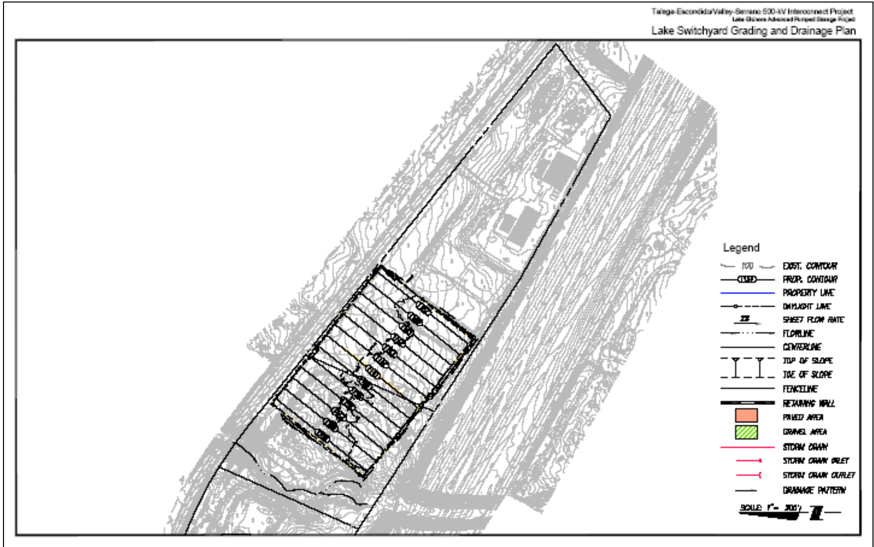
Lake Switchyard Conceptual Grading Plan Source: The Nevada Hydro Company
