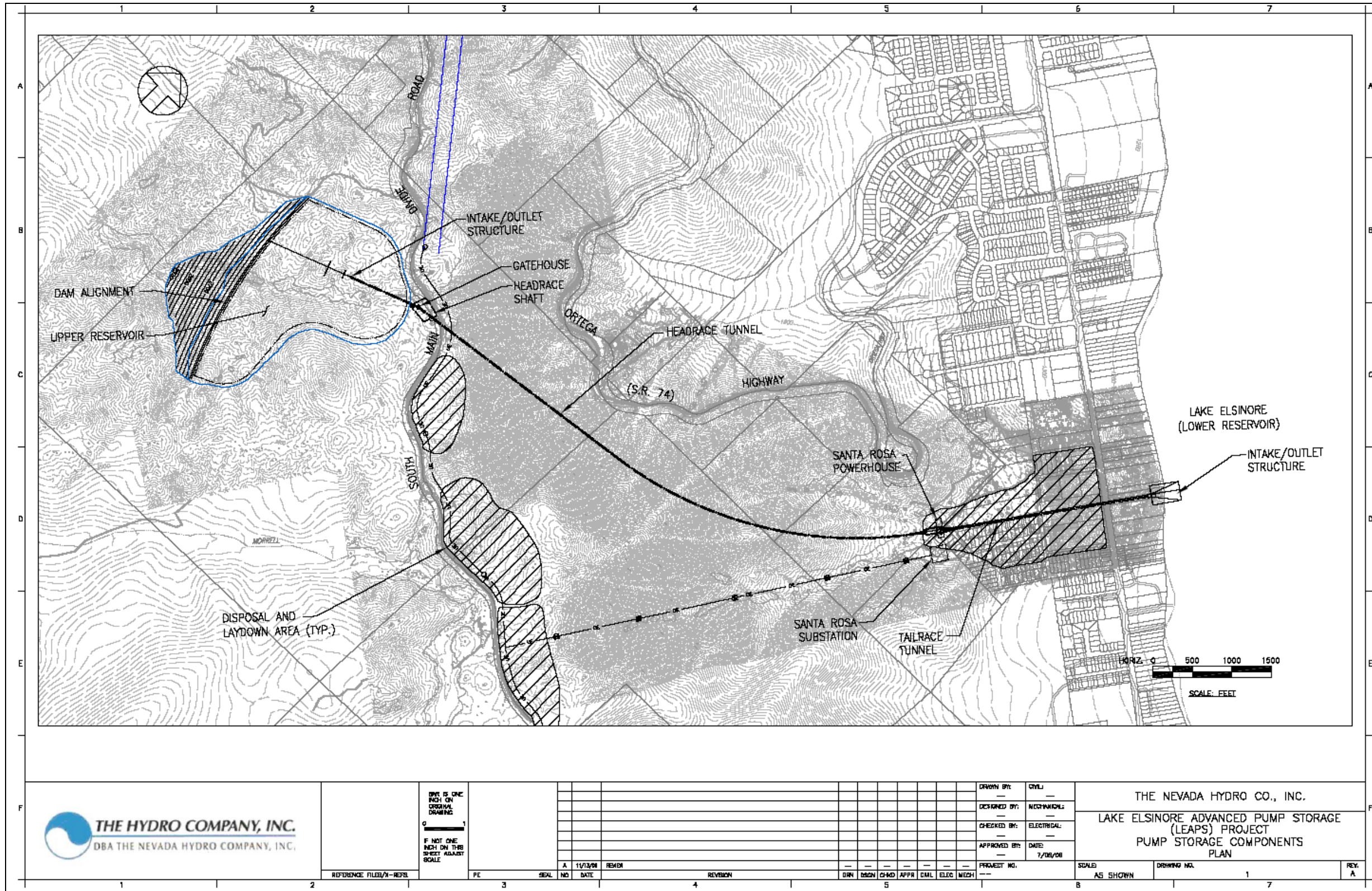
LEAPS Pumped Storage Facility (1 of 2) Source: The Nevada Hydro Company
