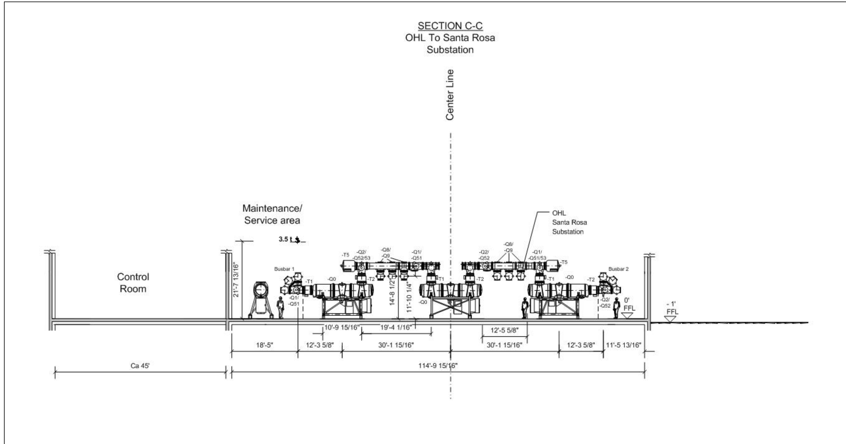
Figure 1.5.1-8: Lake 500 kV Switchyard – Conceptual Elevation Drawings (3 of 3)
