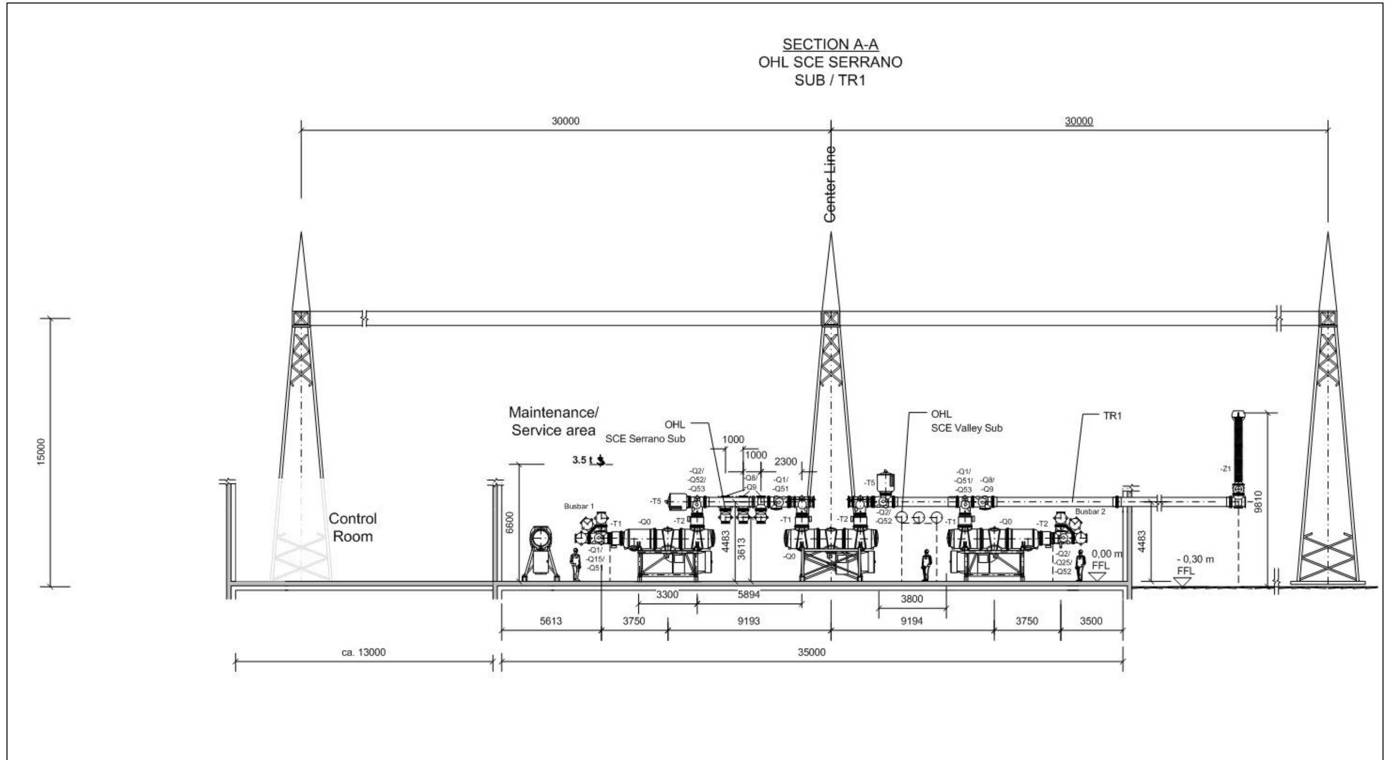
Figure 1.5..1-8: Lake 500 kV Switchyard – Conceptual Elevation Drawings (1 of 3)
