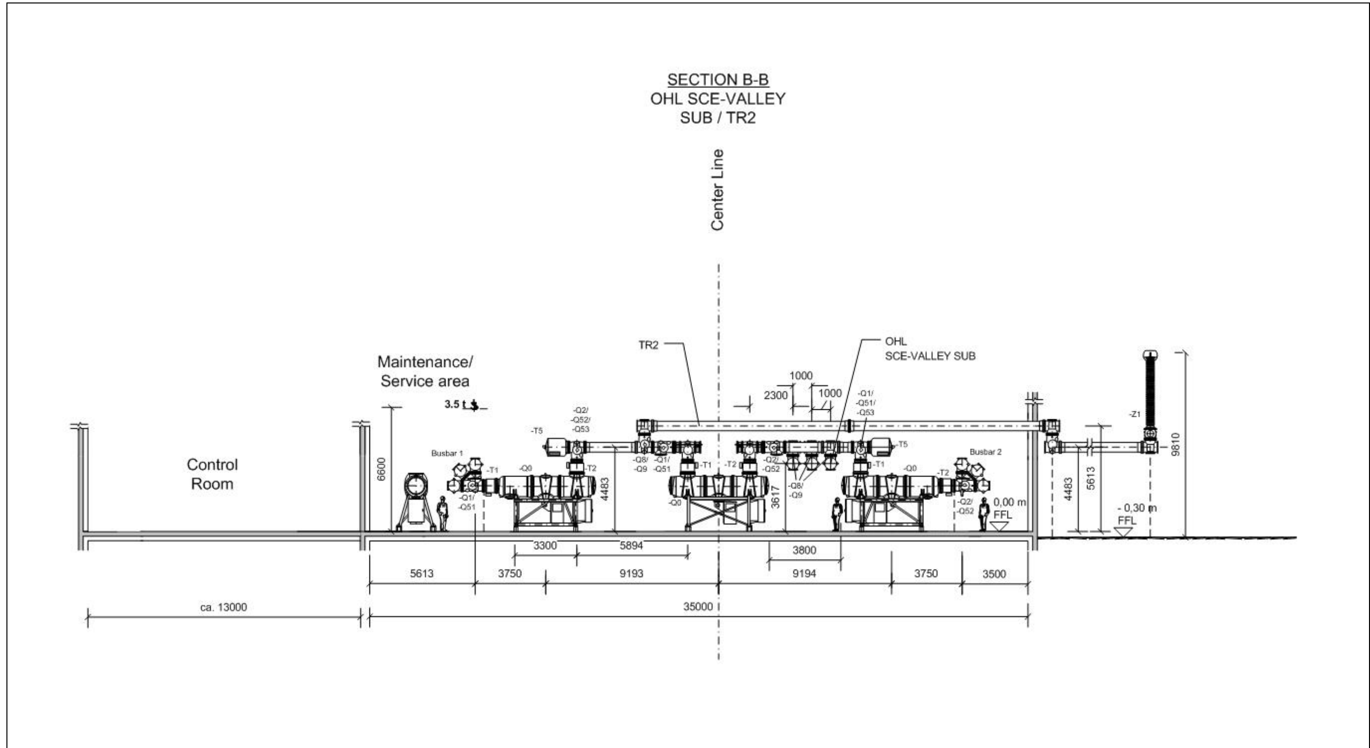
Figure 1.5.1-8: Lake 500 kV Switchyard – Conceptual Elevation Drawings (2 of 3)
