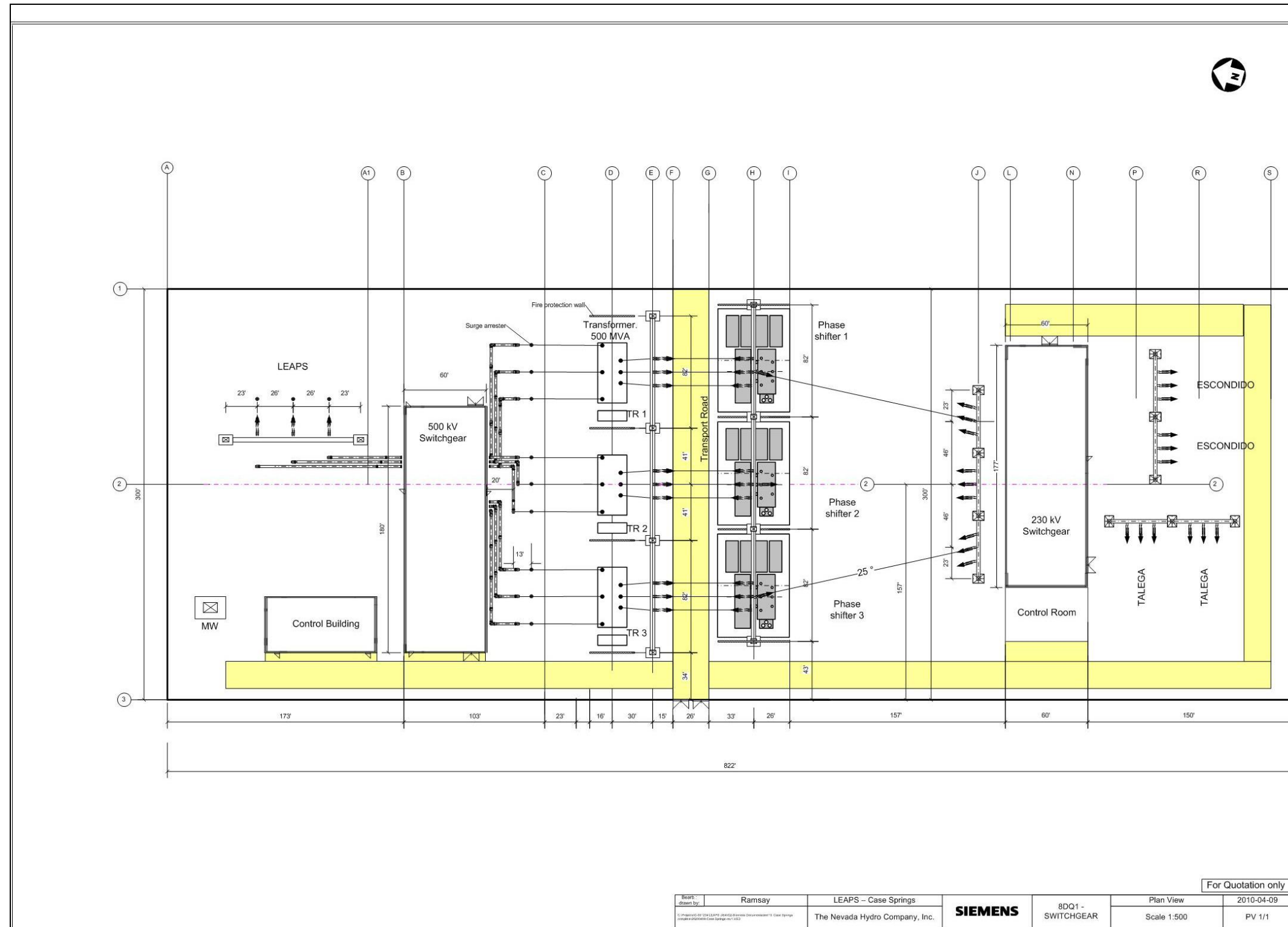
Figure 3.6.1-14 Case Springs Substation – Conceptual Site Plan Source: Siemens Power Transmission & Distribution
