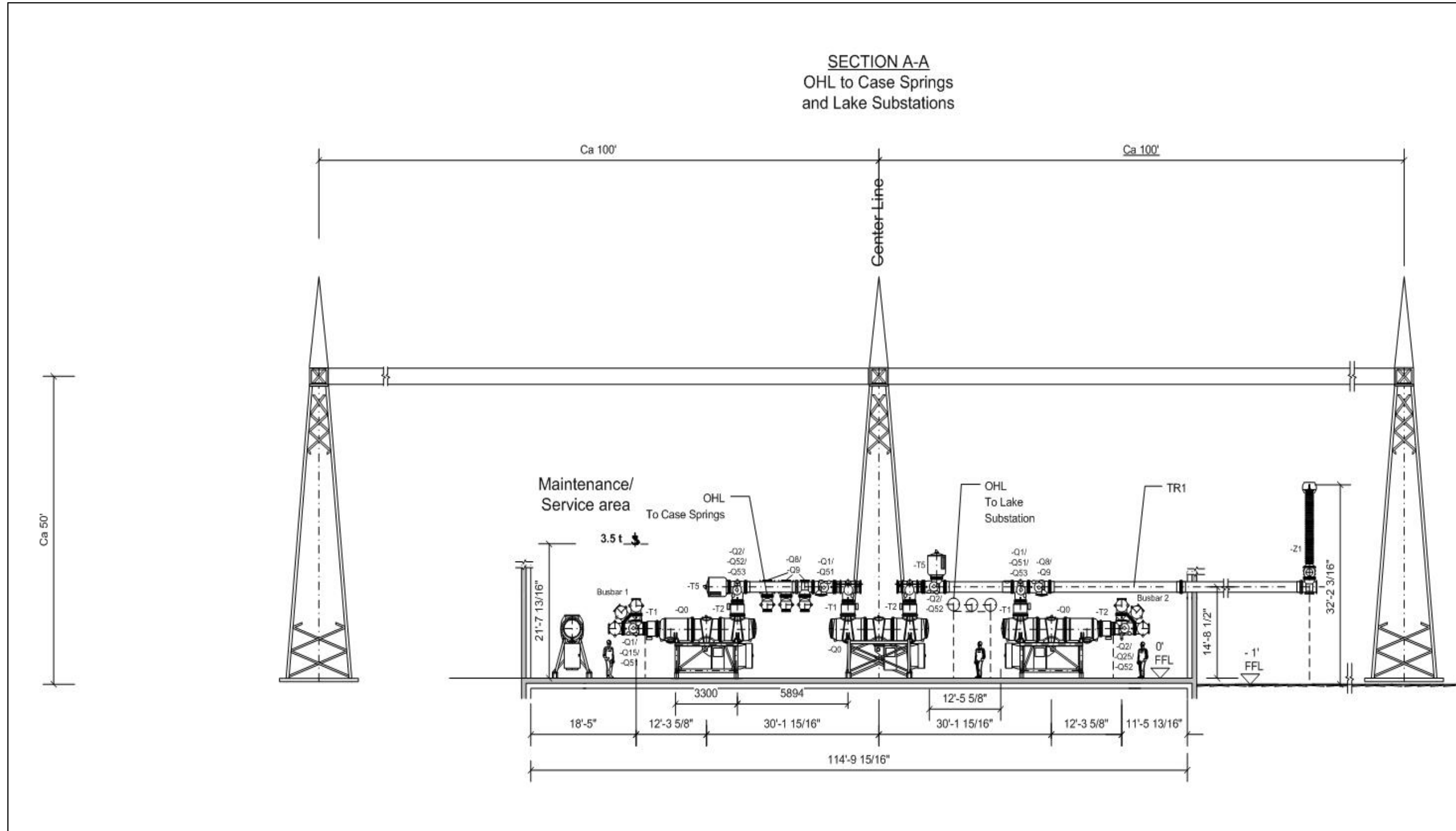
Figure 1.5.1-12: Santa Rosa Substation Site – Conceptual Elevation Drawings (1 of 3)
