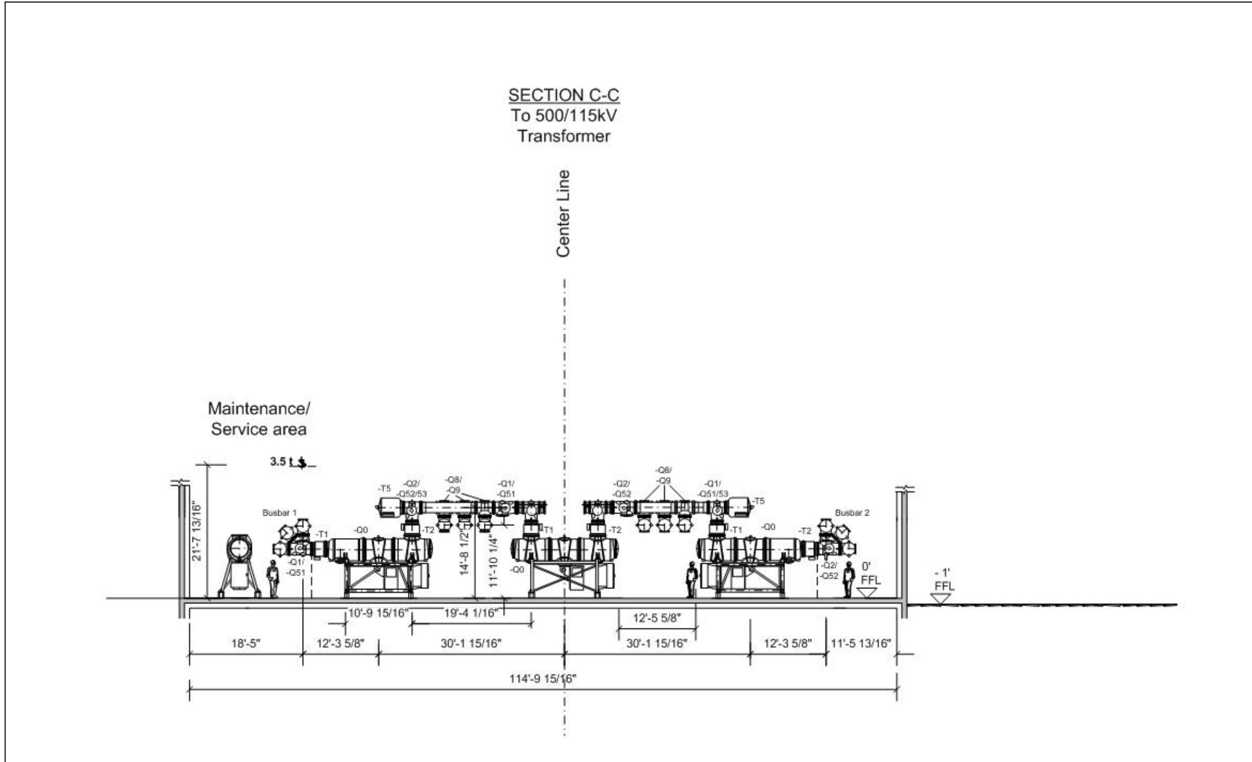
Figure 1.5.1-12: Santa Rosa Substation Site – Conceptual Elevation Drawings (3 of 3)
