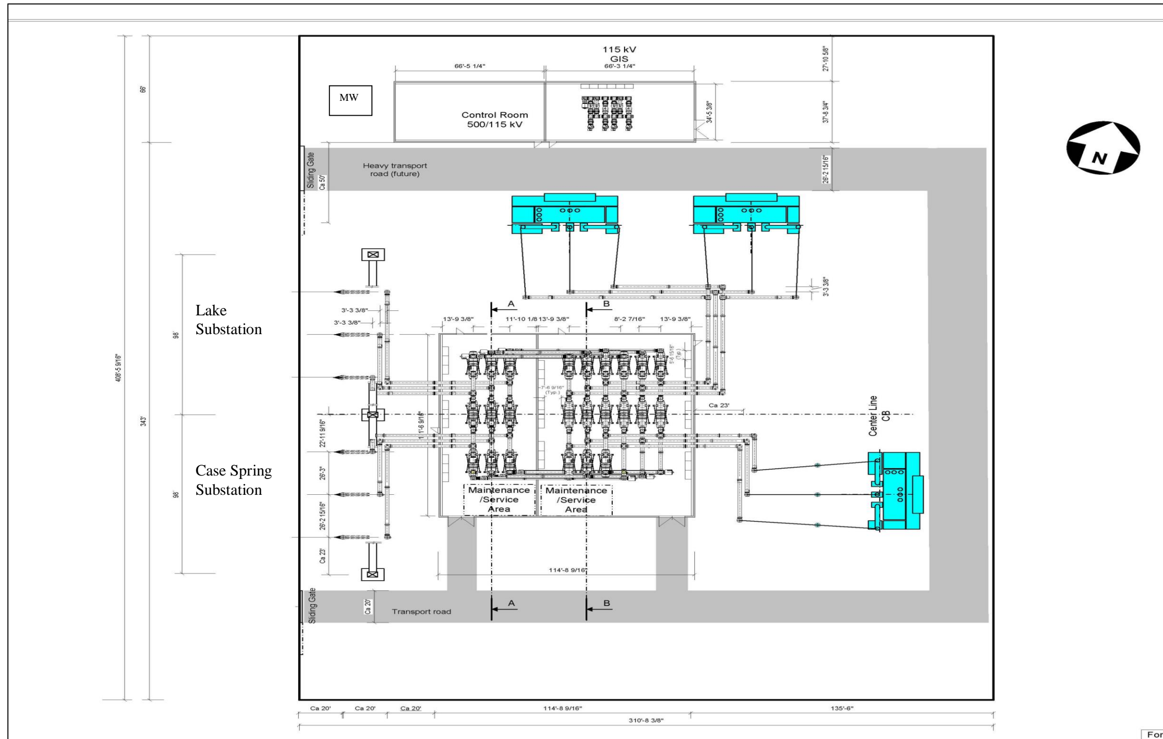
Figure 1.5.1-11: Santa Rosa Substation Site – Conceptual Site Plan Source: Siemens Power Transmission & Distribution
