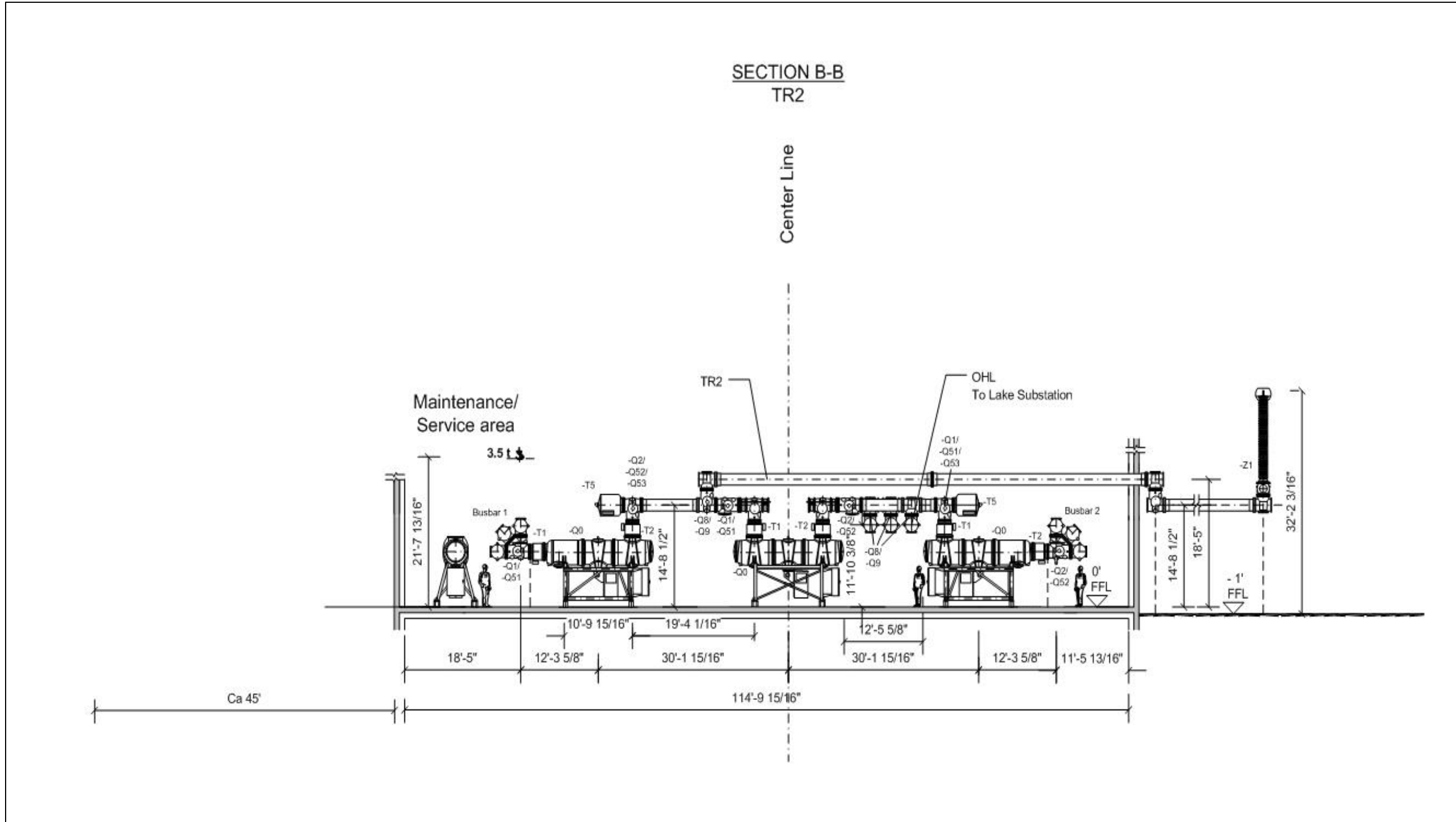
Figure 1.5.1-12: Santa Rosa Substation Site – Conceptual Elevation Drawings (2 of 3)
