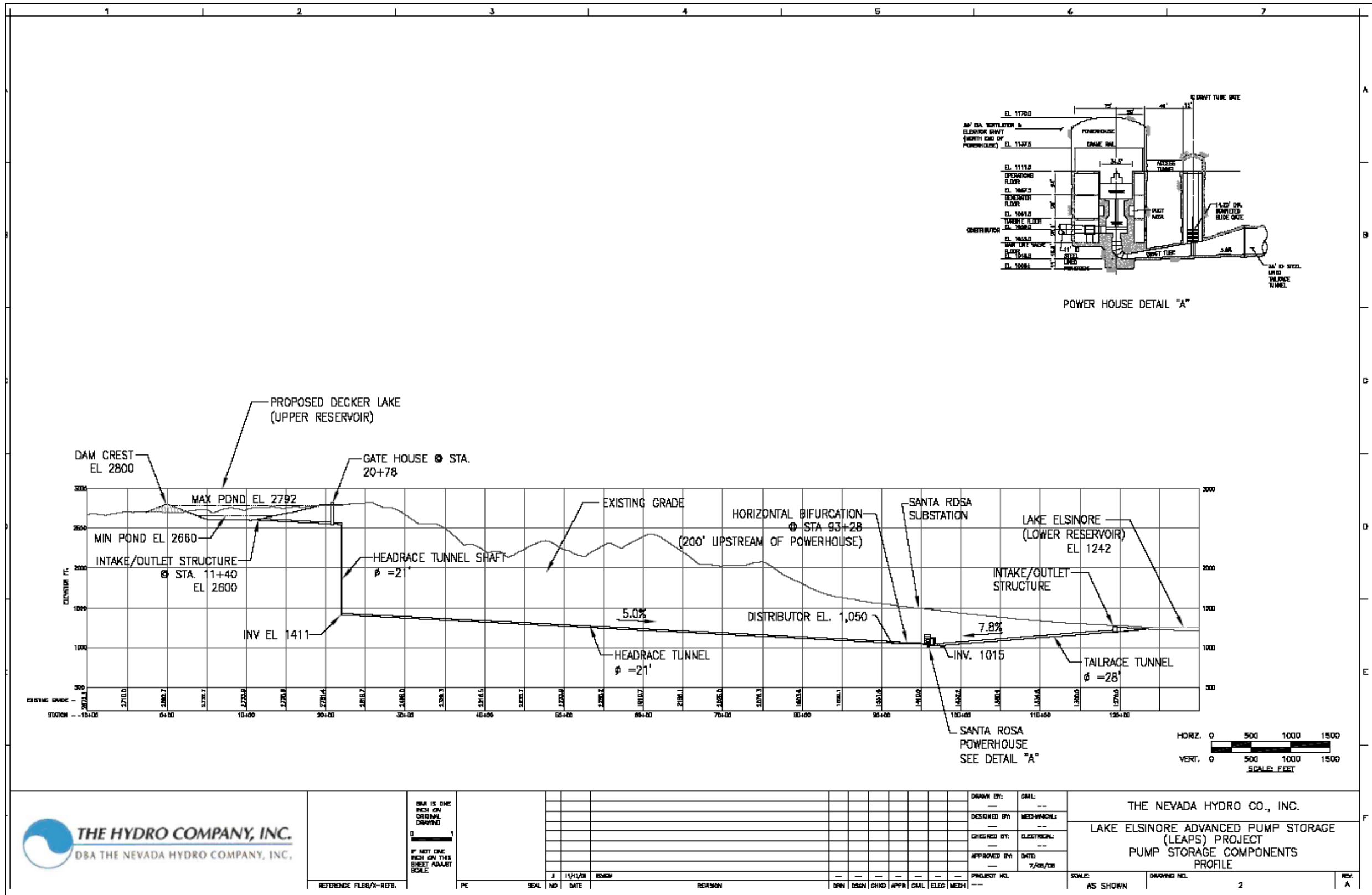
Figure 3.1.1-5: LEAPS Pumped Storage Facility (2 of 2)
